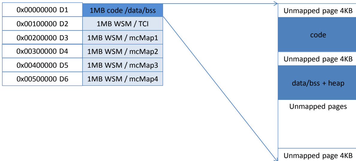
Figure 4: TA Virtual Address Space with legacy layout
