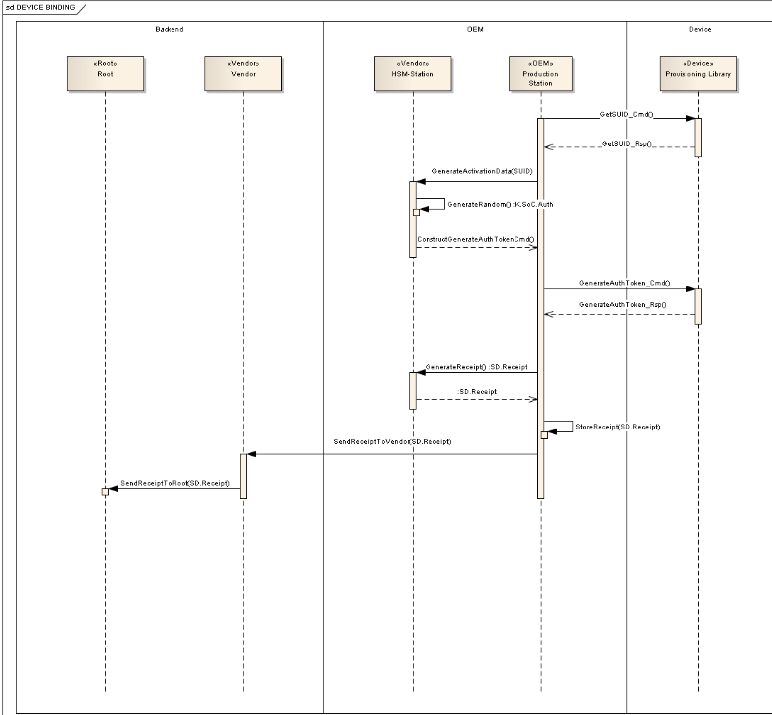
Fig. 1 DEVICE BINDING
