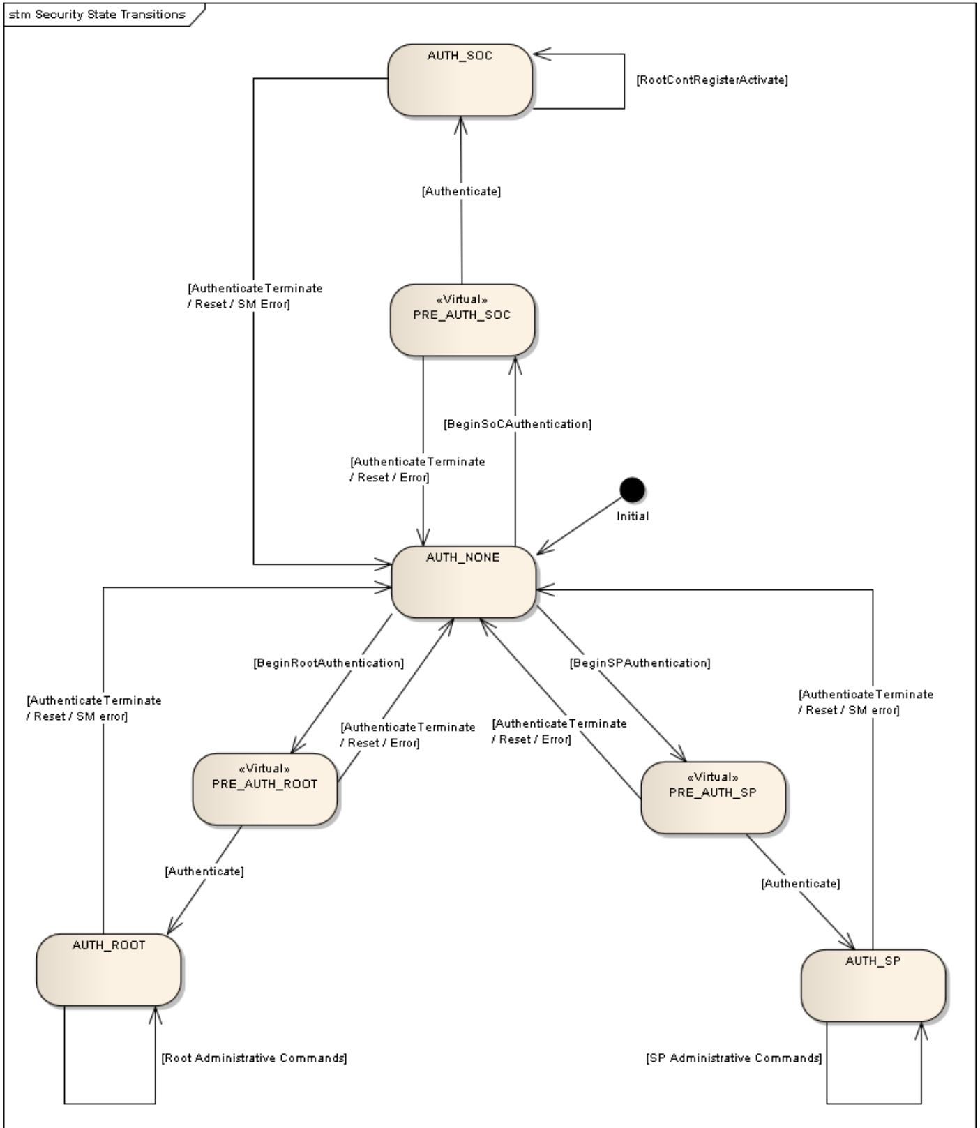
Figure 6: Security State Transitions.
