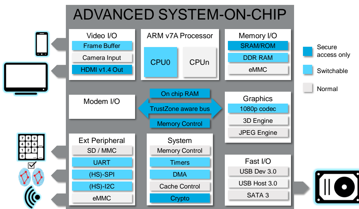
Figure 2: System on Chip with TrustZone.
