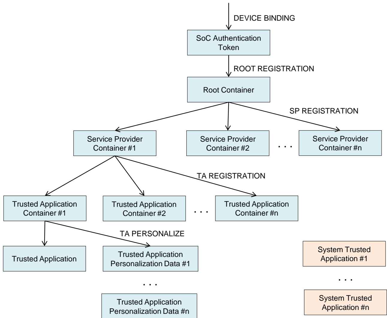
Figure 7: Content Object Hierarchy.
